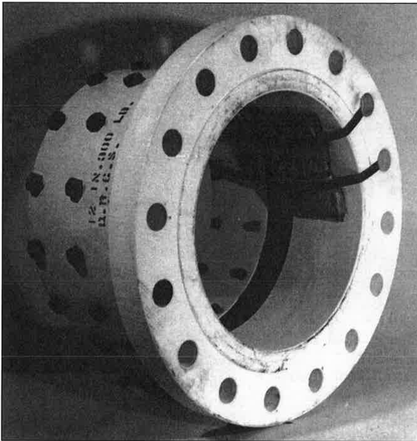
12" 300# Plidco Flange with a double row of clamping screws, for underwater installation.
