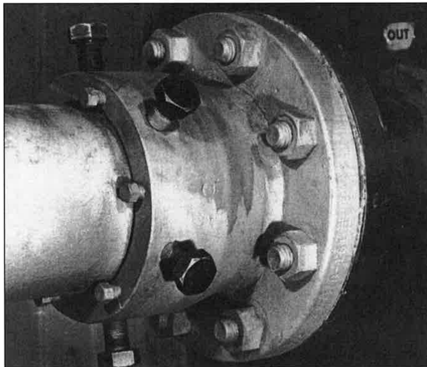
4" 150# Plidco Flange mated to a corresponding flange.
